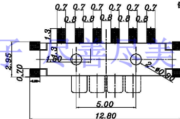
PCB PLERTING PLAN
